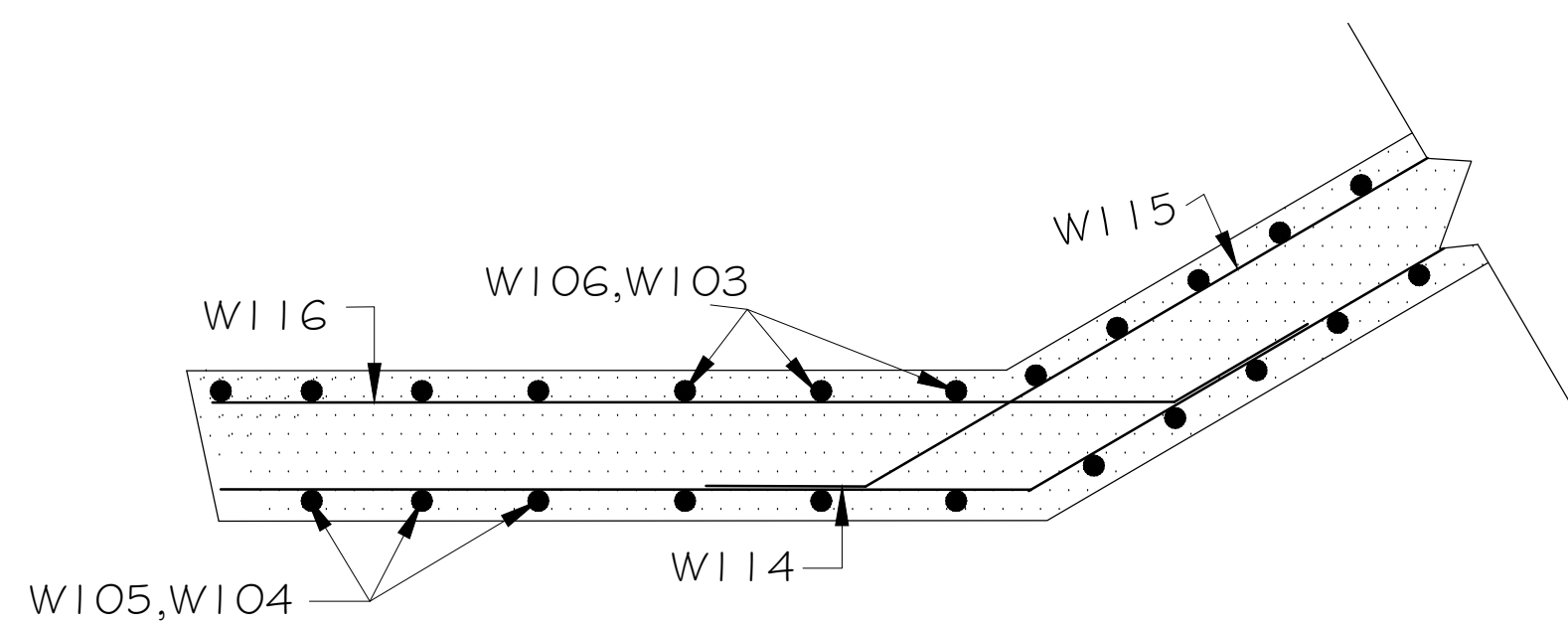
SECTION C
