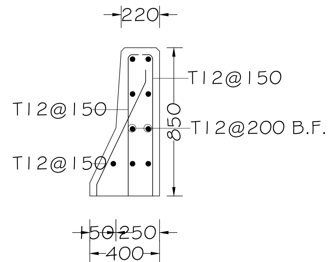
Crush Barrier Reinforcement Scale 1:25
