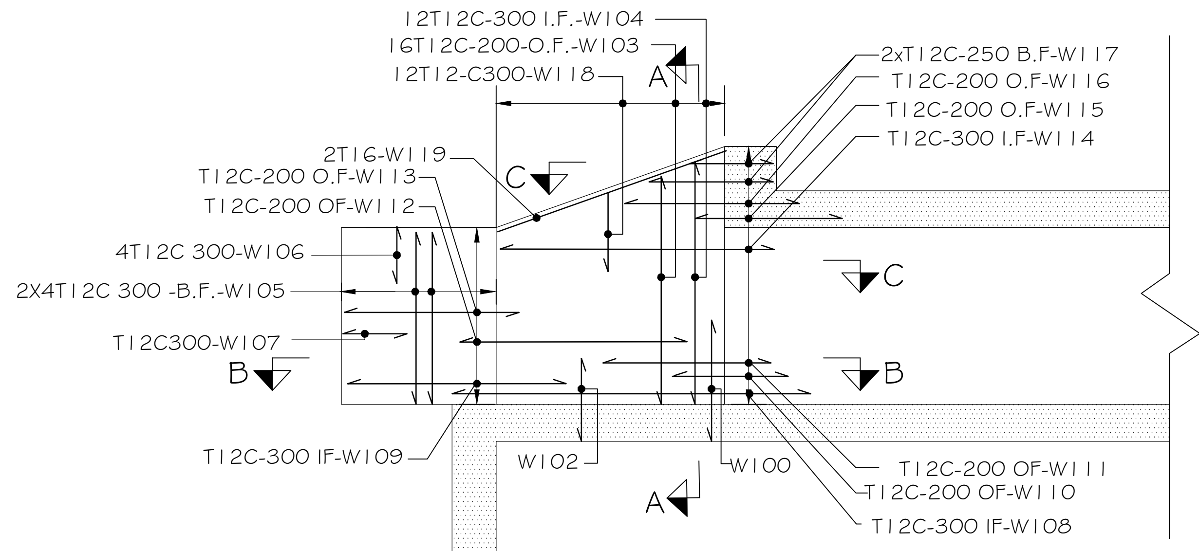
ELEVATION OF WINGWALL, TYPE I
