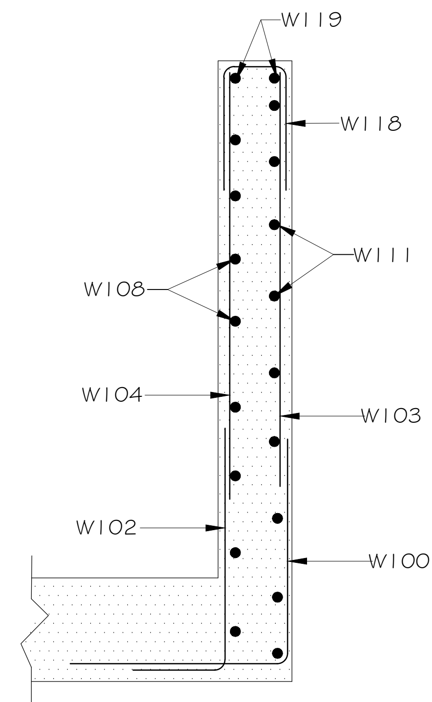
SECTION A
