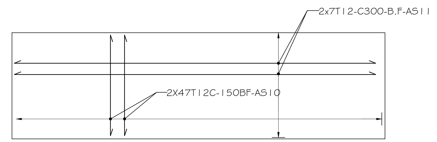
Approach slab
