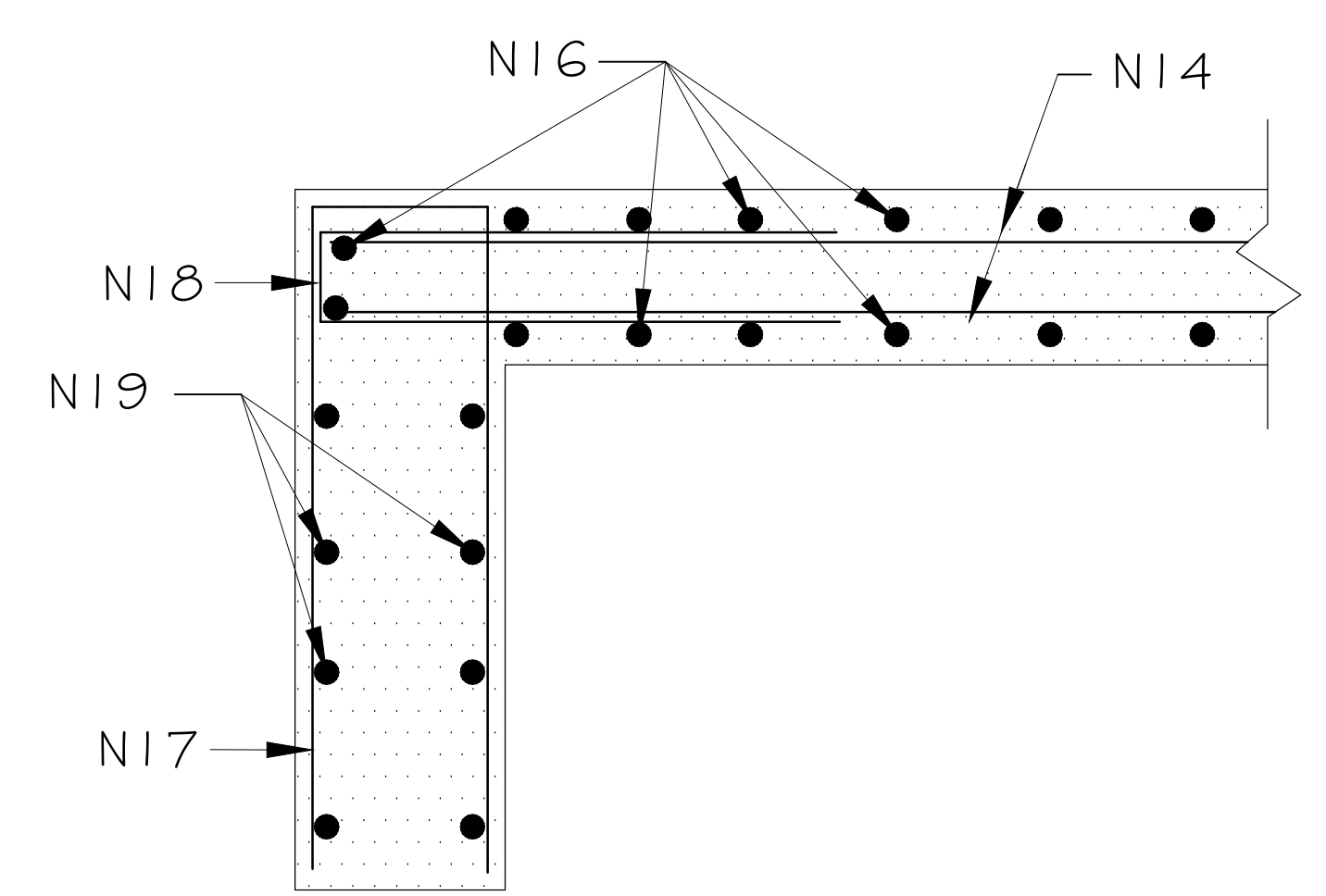
SECTION B
