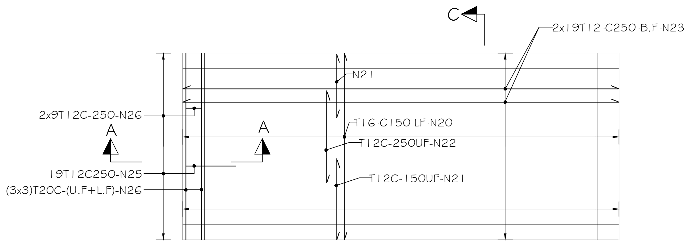
TOP SLAB REINFORCEMENT
