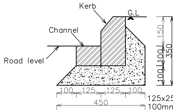
KERB AND CHANNEL (50) 5332'B' SCALE 1:10
