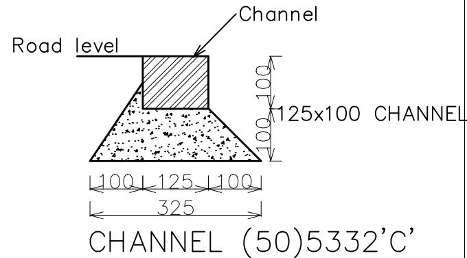
125x250 KERB & 125x100 CHANNEL 100mm Bed & Haunch concrete mix 1:2:4
